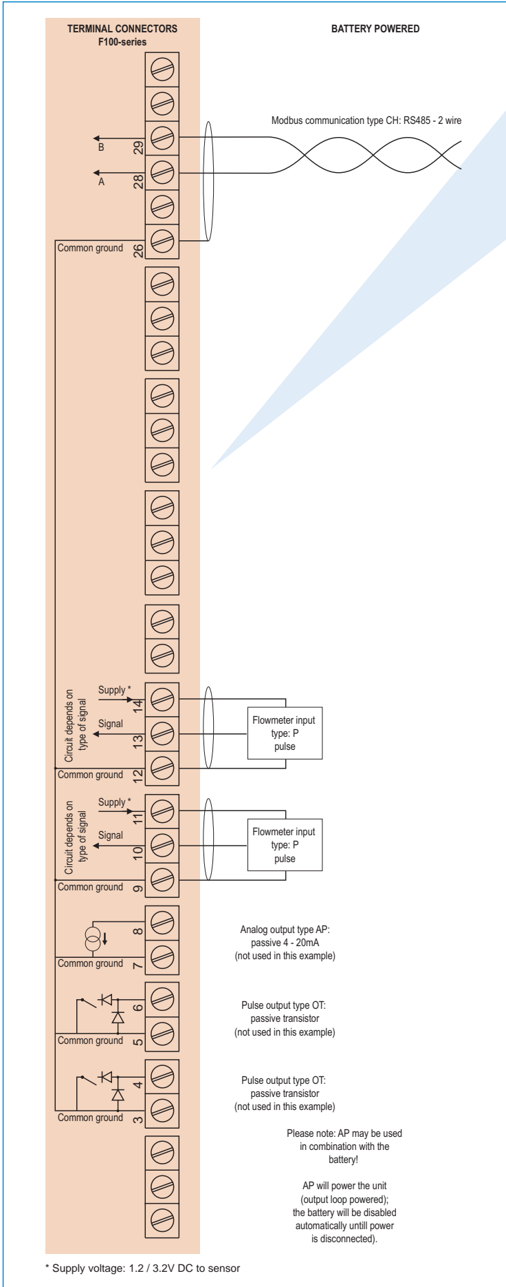
Typical wiring diagram 116-P-(AP)-CH-(OT)-PB
