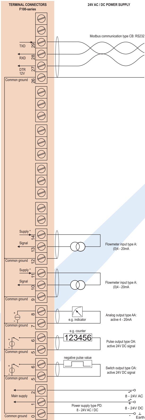
Typical wiring diagram 116-A-AA-CB-OA-PD
