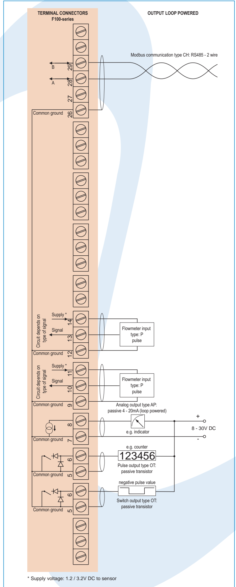
Typical wiring diagram 116-P-AP-CH-OT-PX
