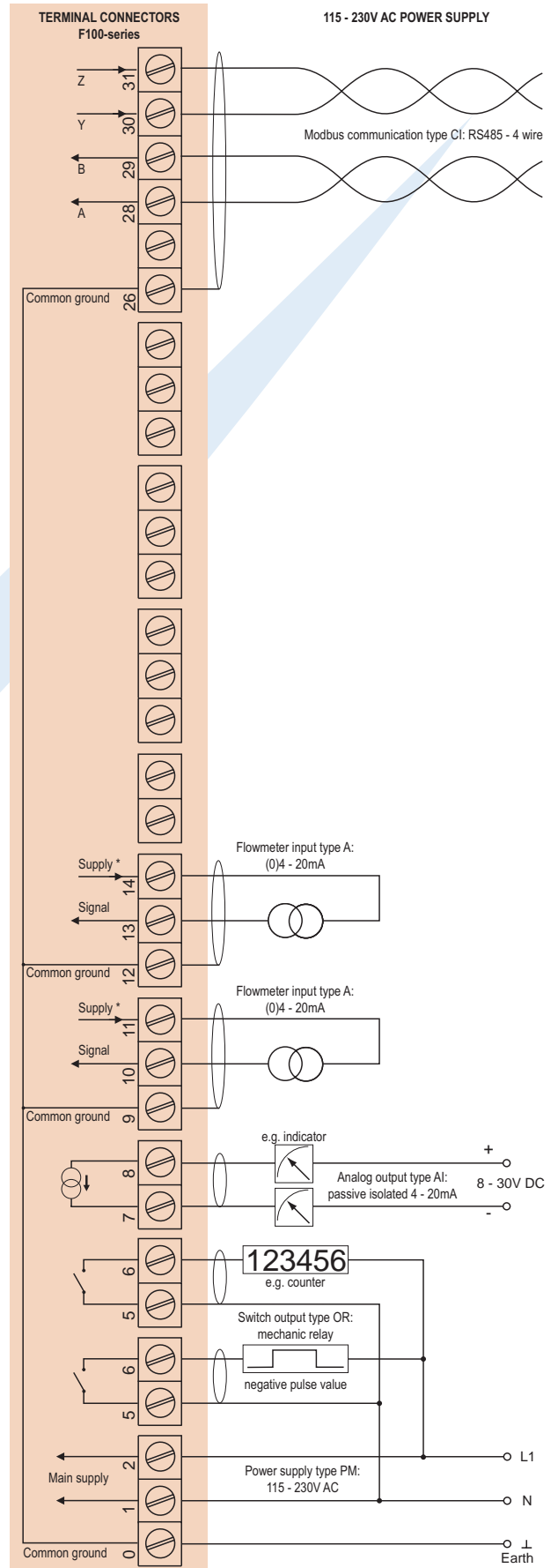
Typical wiring diagram 116-A-AI-CI-OR-PM
